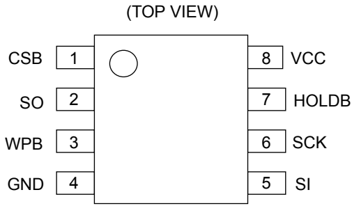
Figure 3. Pin Configuration (SOP-J8, TSSOP-B8)
