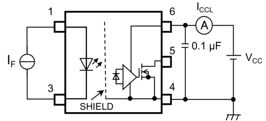
Fig. 12.1.4 I_{CCL} Test Circuit
