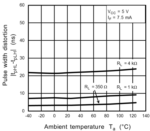
Fig. 12.2.15 |t_{pHL} - t_{pLH}| - T_a
