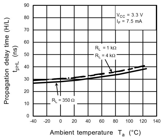
Fig. 12.2.16 t_{pHL} - T_a
