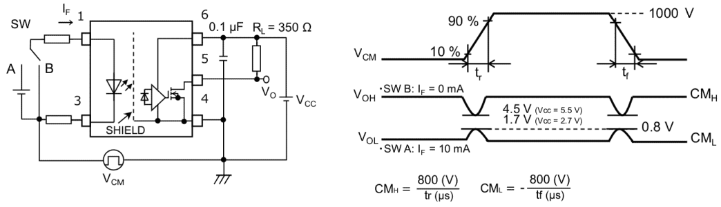
Fig. 12.1.7 Common-Mode Transient Immunity Test Circuit and Waveform
