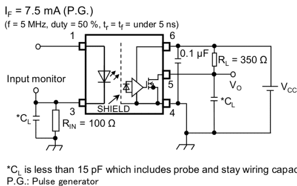
Fig. 12.1.6 Switching Time Test Circuit and Waveform
