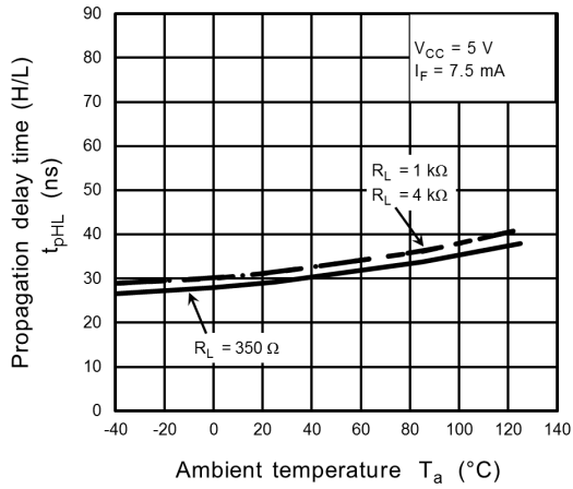
Fig. 12.2.13 t_{pHL} - T_a
