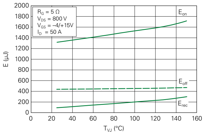
Fig. 17. Typical Switching Energy vs. Junction Temperature
