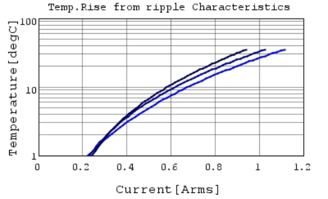
GRM1555C1H270GA01 Temp.rise 500MHz
