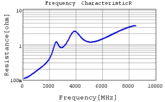
GRM1555C1H560GA01 R DC0V, 25degC
