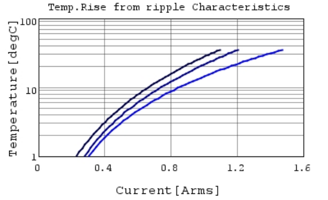
GRM1555C1H560GA01 Temp.rise 200MHz
