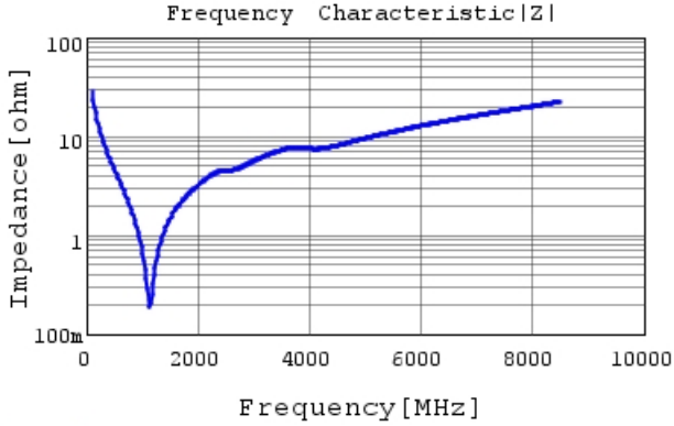
GRM1555C1H560GA01 |Z| DC0V, 25degC
