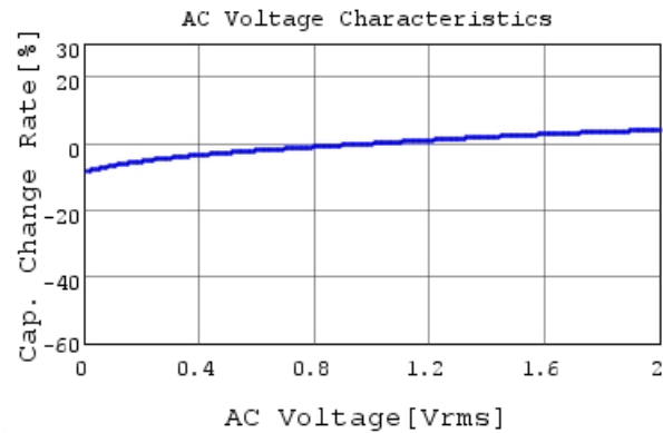
GRM188R61C105KA12 C-AC Voltage capchange, Dc
