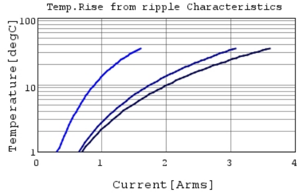
GRM188R61C105KA12 Temp.rise — 100kHz
