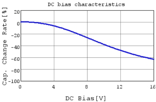
GRM188R61C105KA12 C-DC bias capchange, 25.0c
