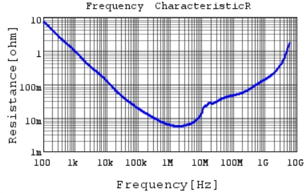
GRM188R61C105KA12 R DCOV,25degC
