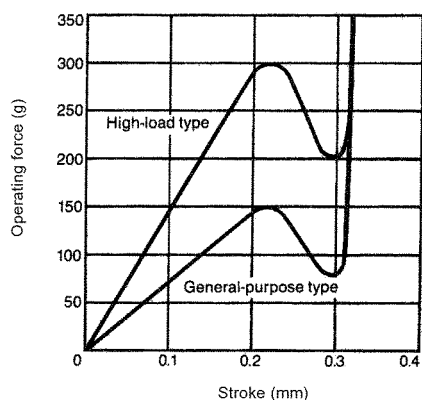
B3W-4□□□ series
