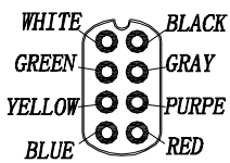
Pin Assignments Front View
