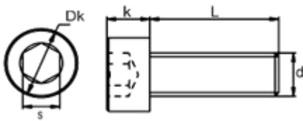
Hex Socket Screw
