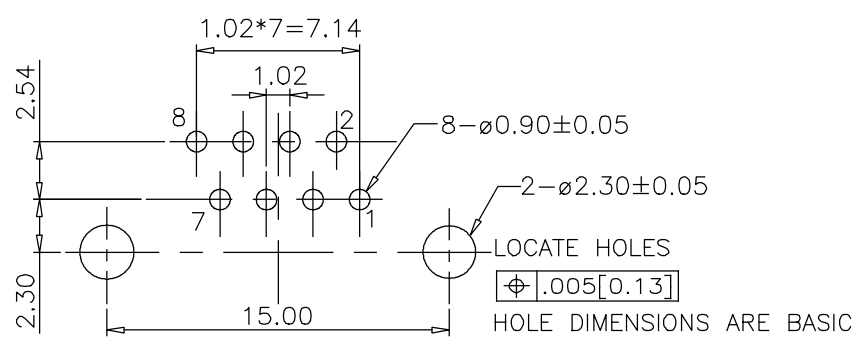
RECOMMENDED P.C.B. LAYOUT (COMPONENT SIDE OF BOARD)
