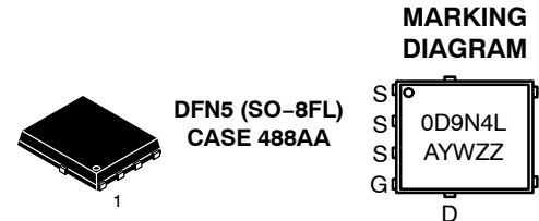
N-CHANNEL MOSFET
