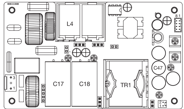
Upper PCB
