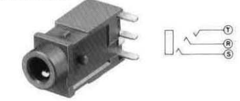
No.M03-749A0 3.5MM STEREO JACK FOR P.C. WATER PROOF
