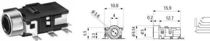
No.MJ-354W-S2 3.5MM STEREO JACK FOR P.C. W/SHIELD HOUSING
