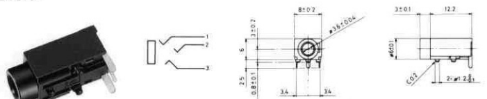
No.M03-681A0 (φ3.5) STEREO
