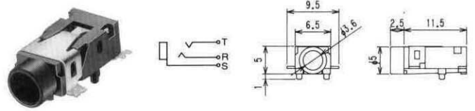
No.M03-292J1 (φ3.5) STEREO
