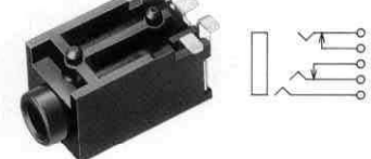
No.MJ-2625 (φ2.5) MONO
