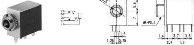
No.MJ-355 (φ3.5) MONO
