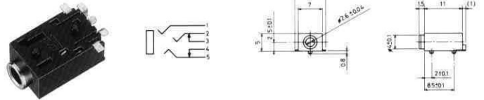
No.M02-641A0 (φ2.5) STEREO
