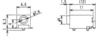
No.MJ-3335-5 (φ3.5) STEREO
