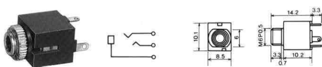
No.MJ-355W (φ3.5) CHASSIS MTG. STEREO JACK
