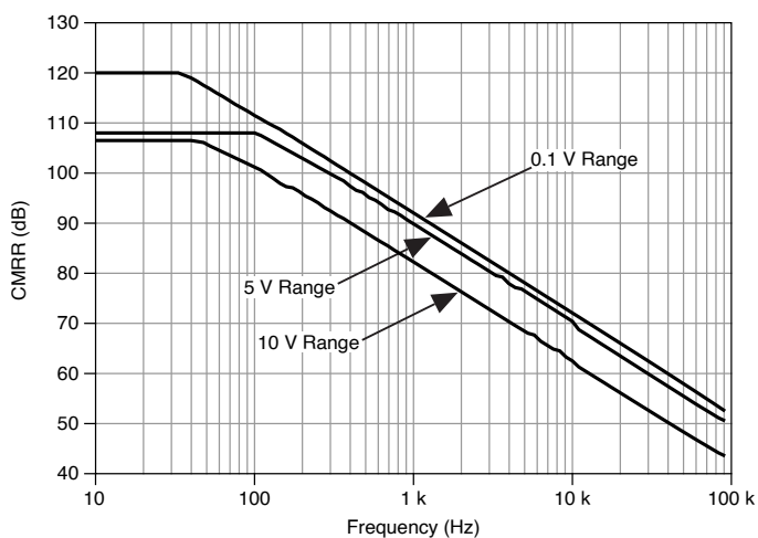
Figure 3. AI <0..31> CMRR
