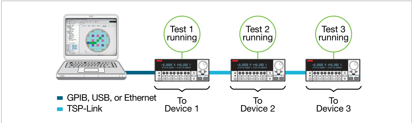
SMU-Per-Pin Parallel Testing using TSP and TSP-Link improves test throughput and lowers the cost of test.
