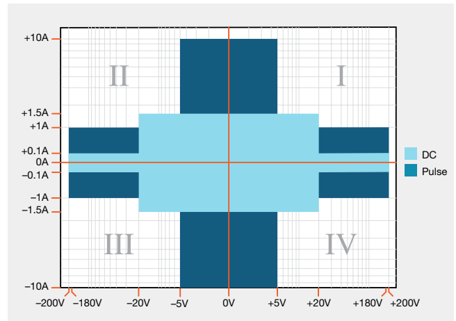
2611B, 2612B, and 2614B I-V capability.
