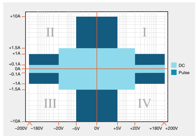
2634B, 2635B, and 2636B I-V capability.
