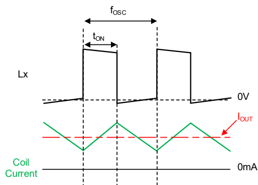
XC9291 series : Example of heavy load operation
