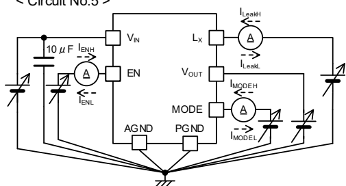
< Circuit No.5 >
