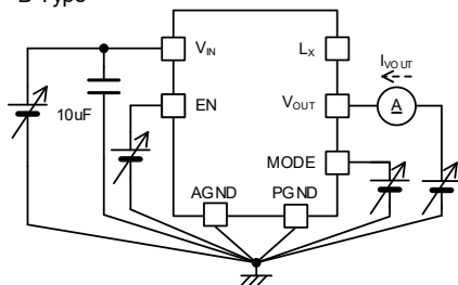
< Circuit No.7 >
