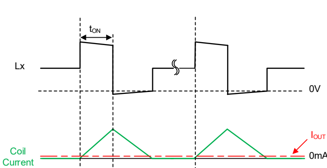
The PWM/PFM control (MODE="L") : Example of light load operation
