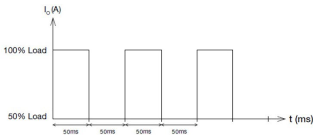
Figure 5. Dynamic Load
