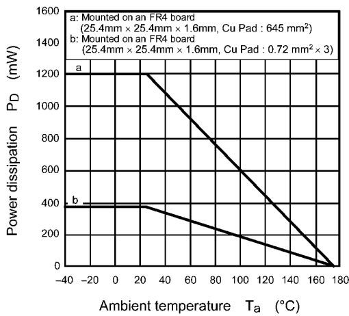
Fig. 8.11 P_D - T_a
