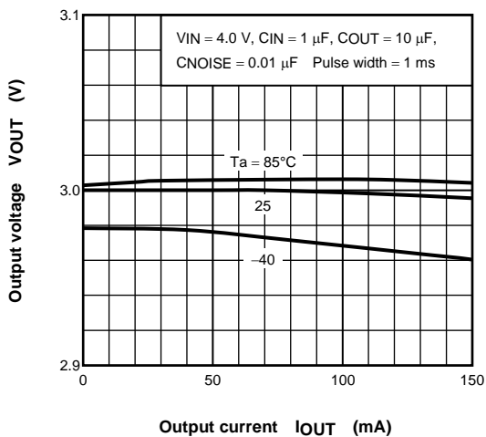
(TAR5SB30) I OUT - V OUT
