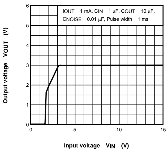
(TAR5SB30) V_{OUT} - V_{IN}
