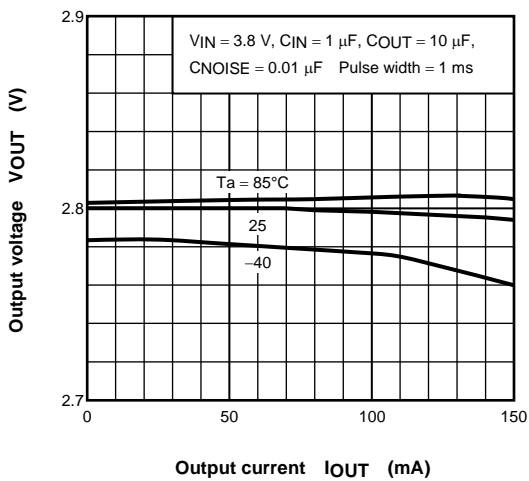
(TAR5SB28) I OUT - V OUT
