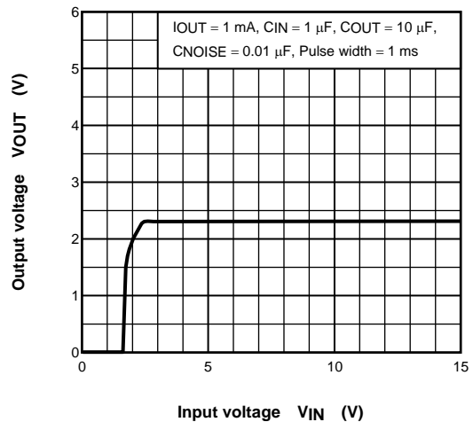
(TAR5SB23) V_{OUT} - V_{IN}
