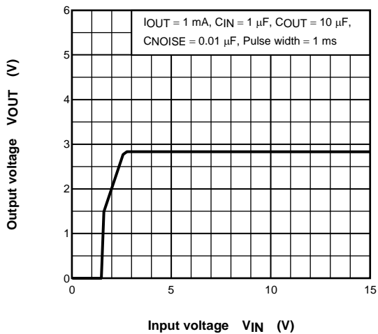
(TAR5SB29) V_{OUT} - V_{IN}
