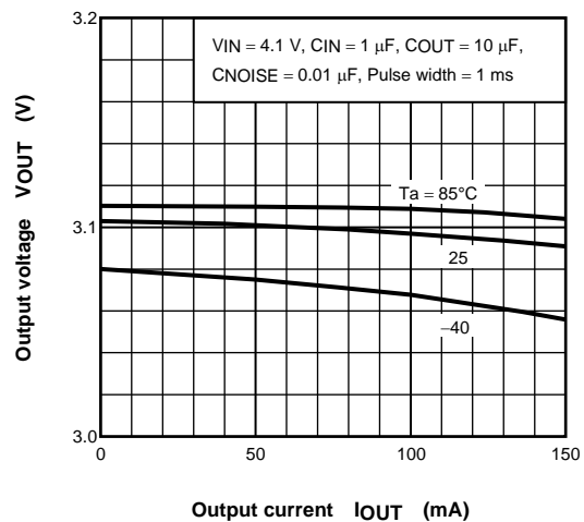
(TAR5SB31) I OUT - V OUT
