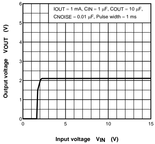
(TAR5SB21) V_{OUT} - V_{IN}
