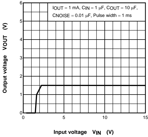
(TAR5SB15) V_{OUT} - V_{IN}
