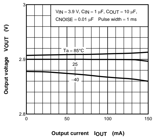
(TAR5SB29) I OUT - V OUT
