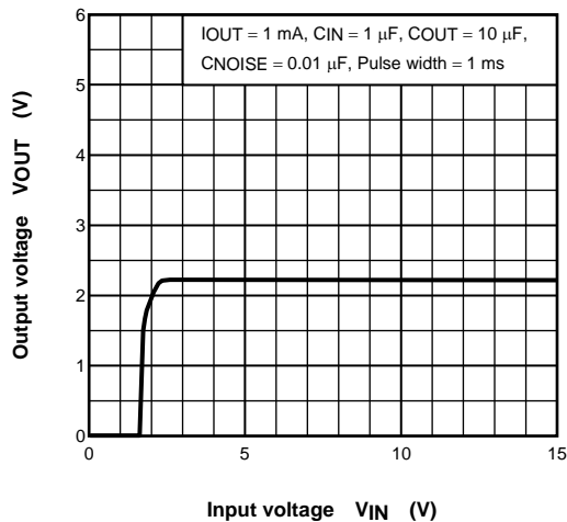
(TAR5SB22) V_{OUT} - V_{IN}
