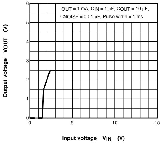
(TAR5SB25) V_{OUT} - V_{IN}
