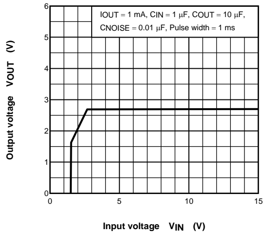
(TAR5SB27) V_{OUT} - V_{IN}
