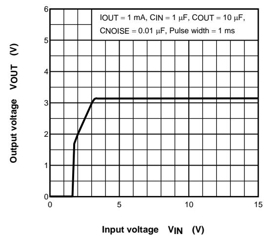
(TAR5SB31) V_{OUT} - V_{IN}
