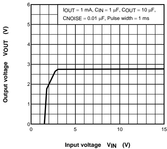
(TAR5SB28) V_{OUT} - V_{IN}
