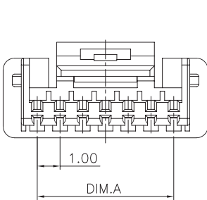
4 to 9 Circuits
