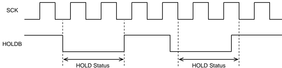
Figure 39. HOLD Status
