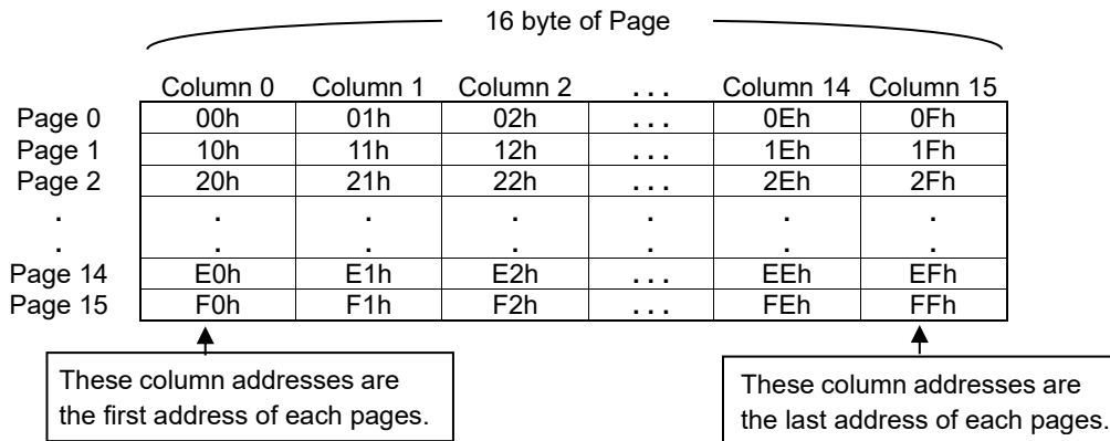
Figure 45. EEPROM physical address for Page Write command (16 Byte)
