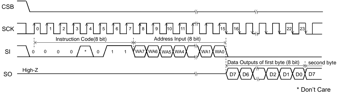
Figure 42. Read Command
