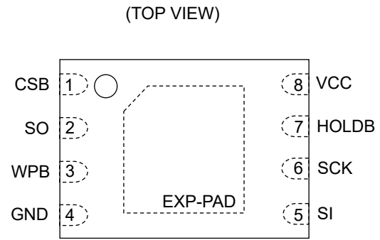
Figure 3-(b). Pin Configuration (VSON08AX2030)
