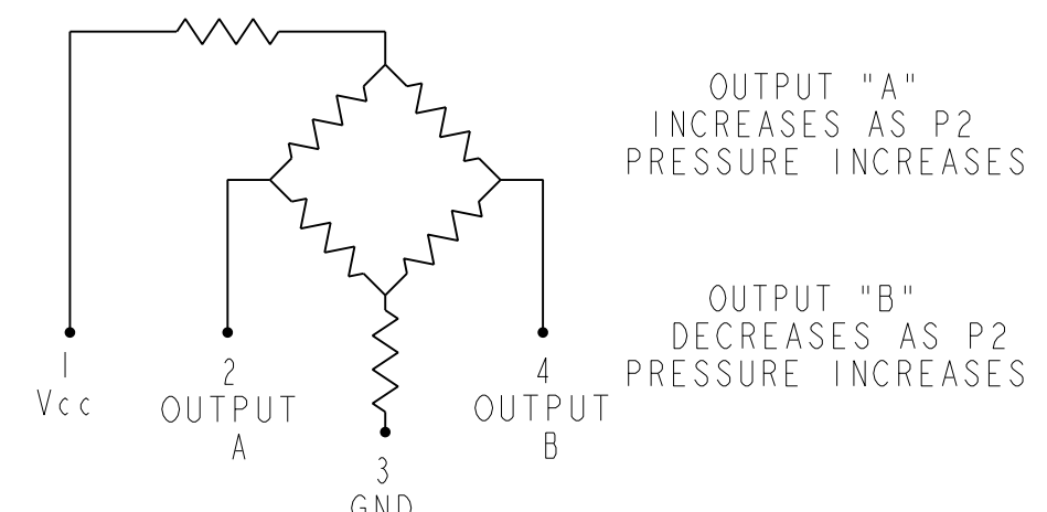
CIRCUIT DIAGRAM
