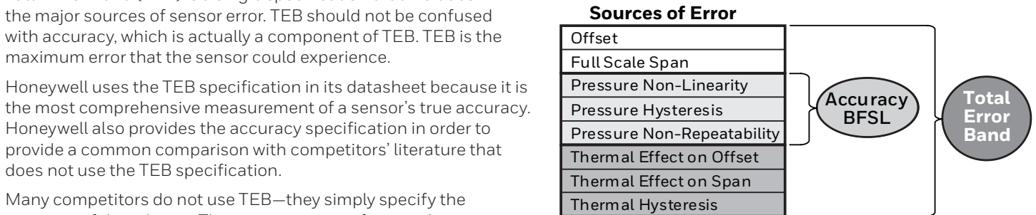
FIGURE 4. TEB COMPONENTS FOR THE MIP SERIES
