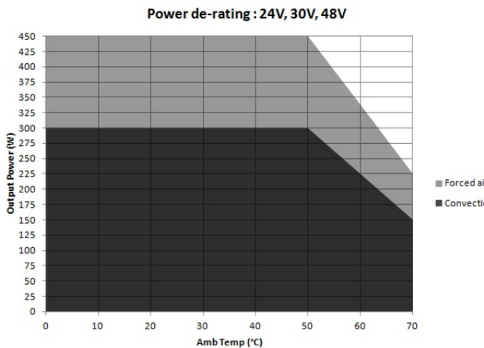
Figure 1. Derating Curves
