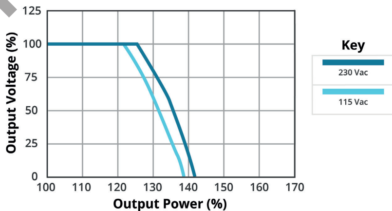
TYPICAL OVER CURRENT PROTECTION CURVE (PDRC-75-24)
