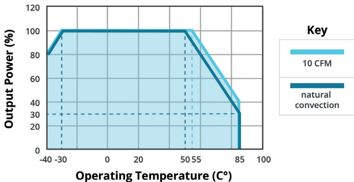
TEMPERATURE DERATING CURVE (open-frame versions)
