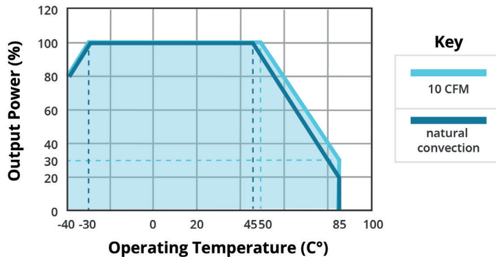
TEMPERATURE DERATING CURVE (-CNF versions)
