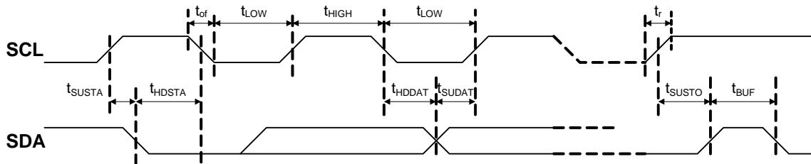
Figure 15. PC / SMBus Timing
