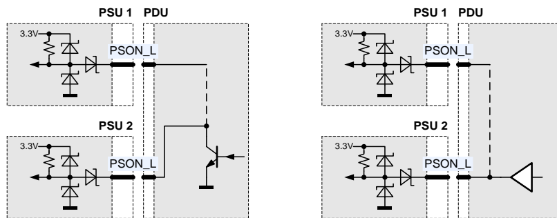
Figure 16. PSON_L connection
