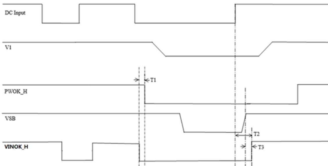
Figure 13. VINOK_H Timing
