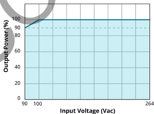
INPUT VOLTAGE DERATING CURVE
