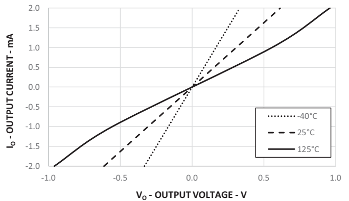
Figure 6: Output Current vs. Output Voltage
