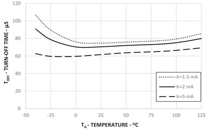
Figure 10: Turn-Off Time vs. Temperature (Test Condition: V_{DD} = 40\text{V} , R_{LOAD} = 20 \text{ k}\Omega )
