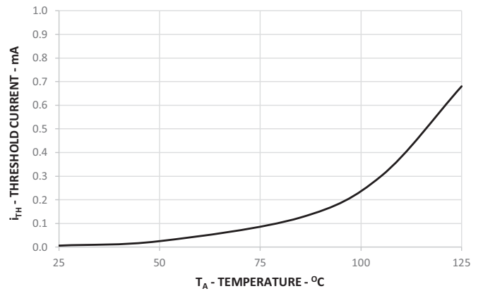
Figure 2: LED Forward Current Threshold vs Temperature
