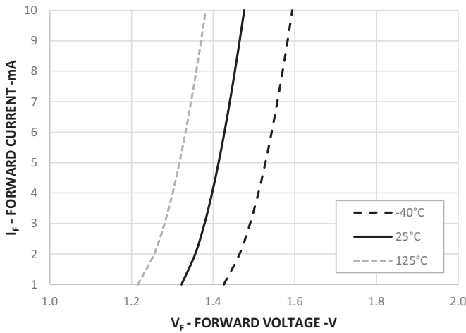
Figure 1: LED Forward Current vs. LED Forward Voltage
