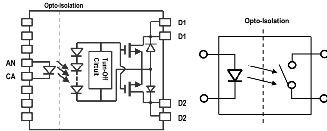
Figure 13: Equivalent Relay Diagram
