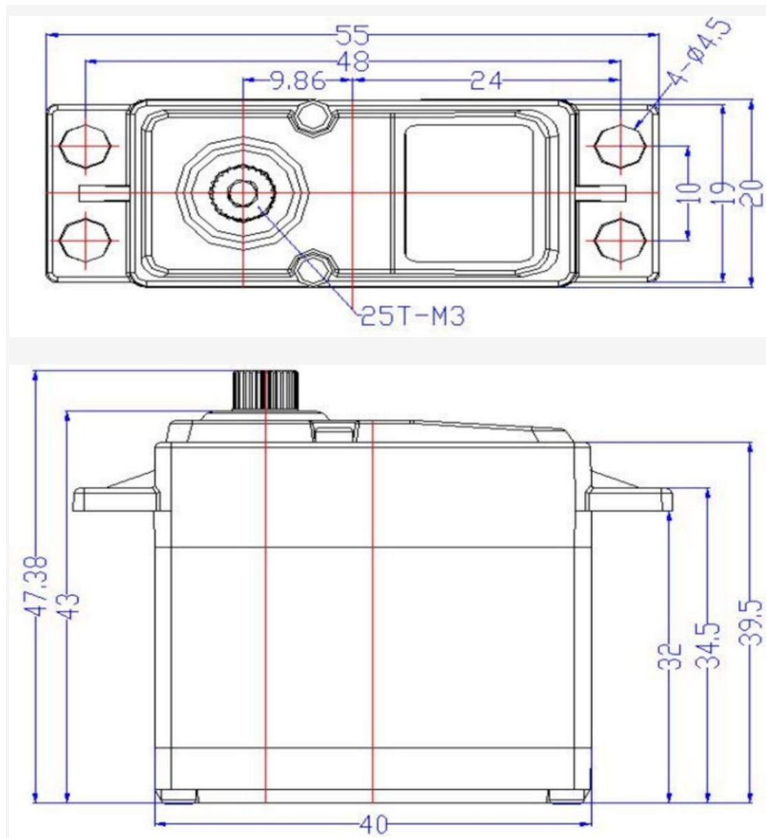
Dimensional Diagram
