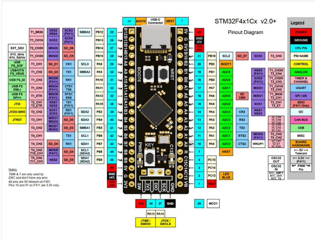
Pinout Diagram
