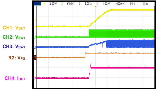
Start-Up through EN I_{OUT} = 1A, \text{MODE/SYNC is high}
