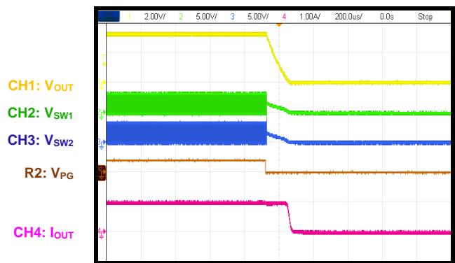
Shutdown through EN I_{OUT} = 1A, \text{MODE/SYNC is high}
