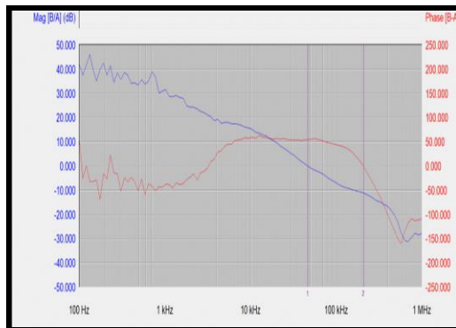
Bode Plot V_{IN} = 3.3V, V_{OUT} = 3.6V, I_{OUT} = 0.05A, \text{MODE/SYNC is high}
