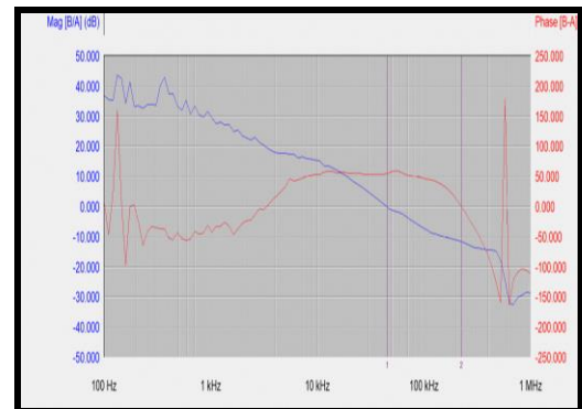
Bode Plot V_{IN} = 3.3V, V_{OUT} = 3.6V, I_{OUT} = 1A, \text{MODE/SYNC is high}
