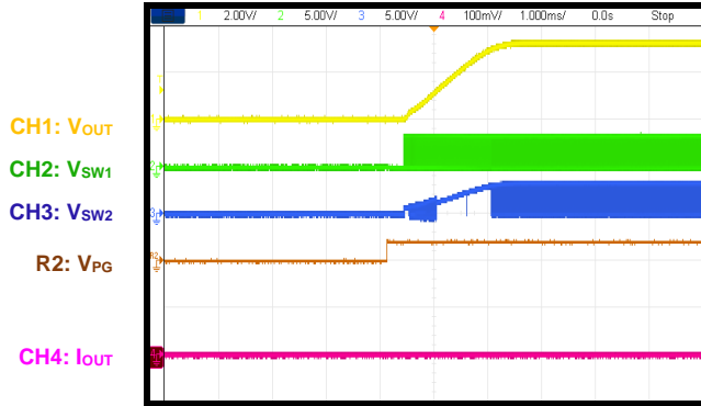
Start-Up through EN I_{OUT} = 0A, \text{MODE/SYNC is high}
