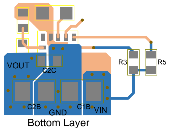
Figure 3: Recommended PCB Layout
