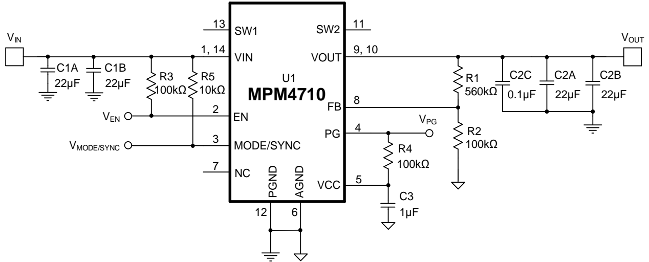
Figure 4: Typical Application Circuit ( V_{OUT} = 3.3V )
