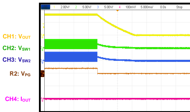
Shutdown through EN I_{OUT} = 0.01A, \text{MODE/SYNC is high}
