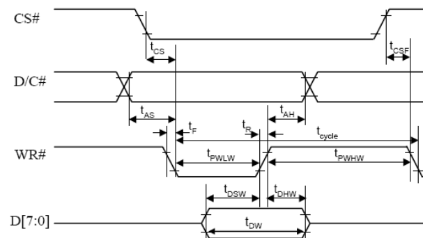
( Write Timing )
