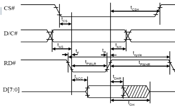
( Read Timing )
