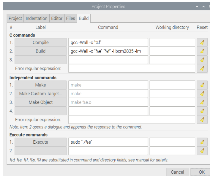
FIGURE 7 - BUILD COMMANDS SETUP
