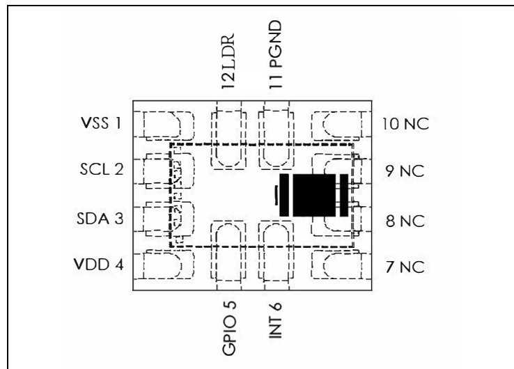
Figure 3: Pin Diagram of TCS3707
