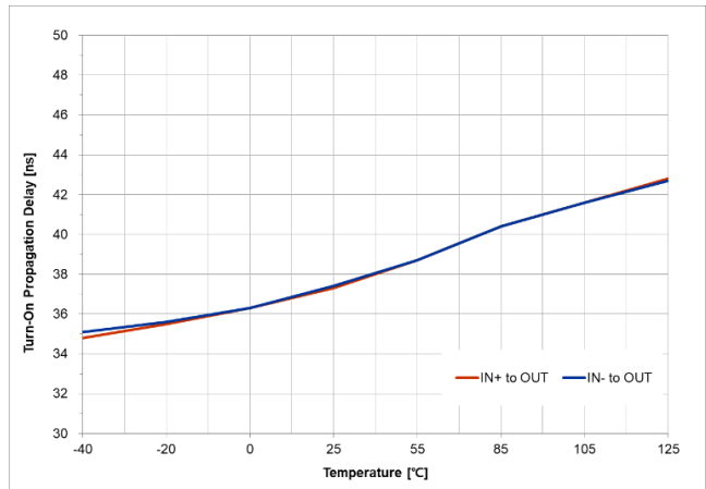
Figure 45. Turn-on Propagation Delay vs. Temperature (C LOAD = 0 nF)
