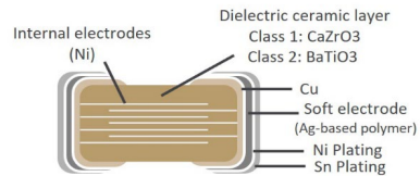
AS Series construction
