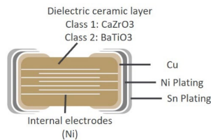
AC series construction
