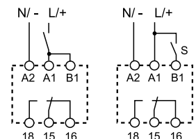
Wiring diagram (without control signal)
