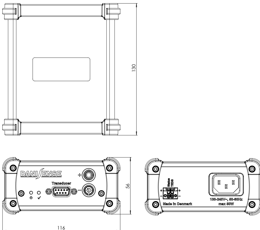
Figure 3: Box dimensions
