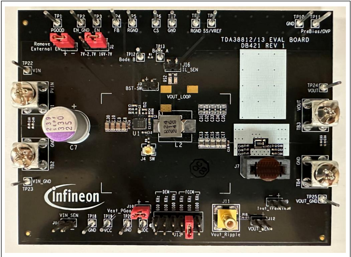
Figure 1 Evaluation board
