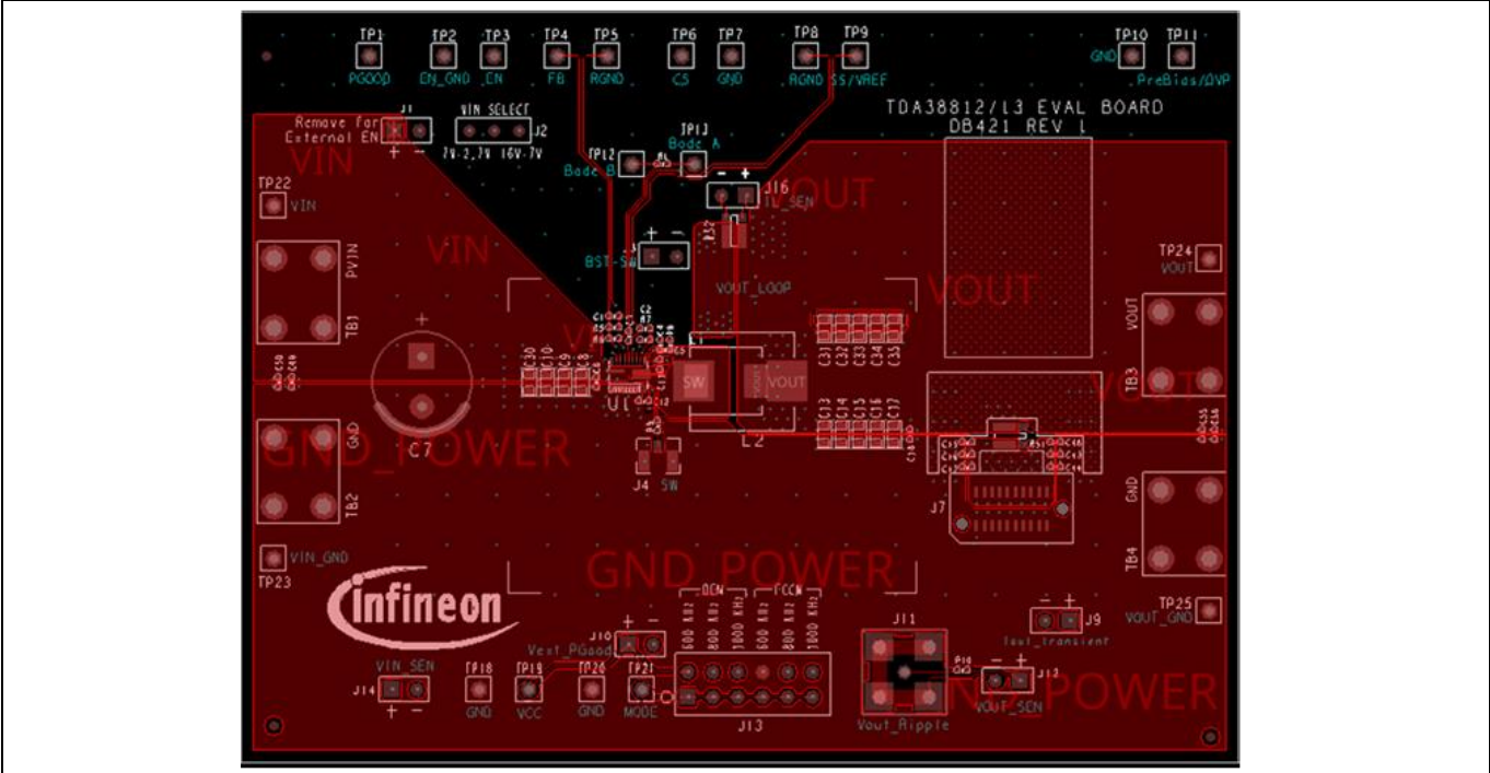
Figure 2 Top layer
