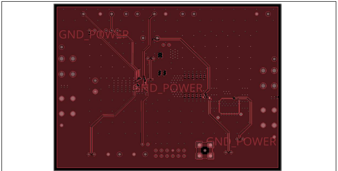
Figure 5 Inner layer 2
