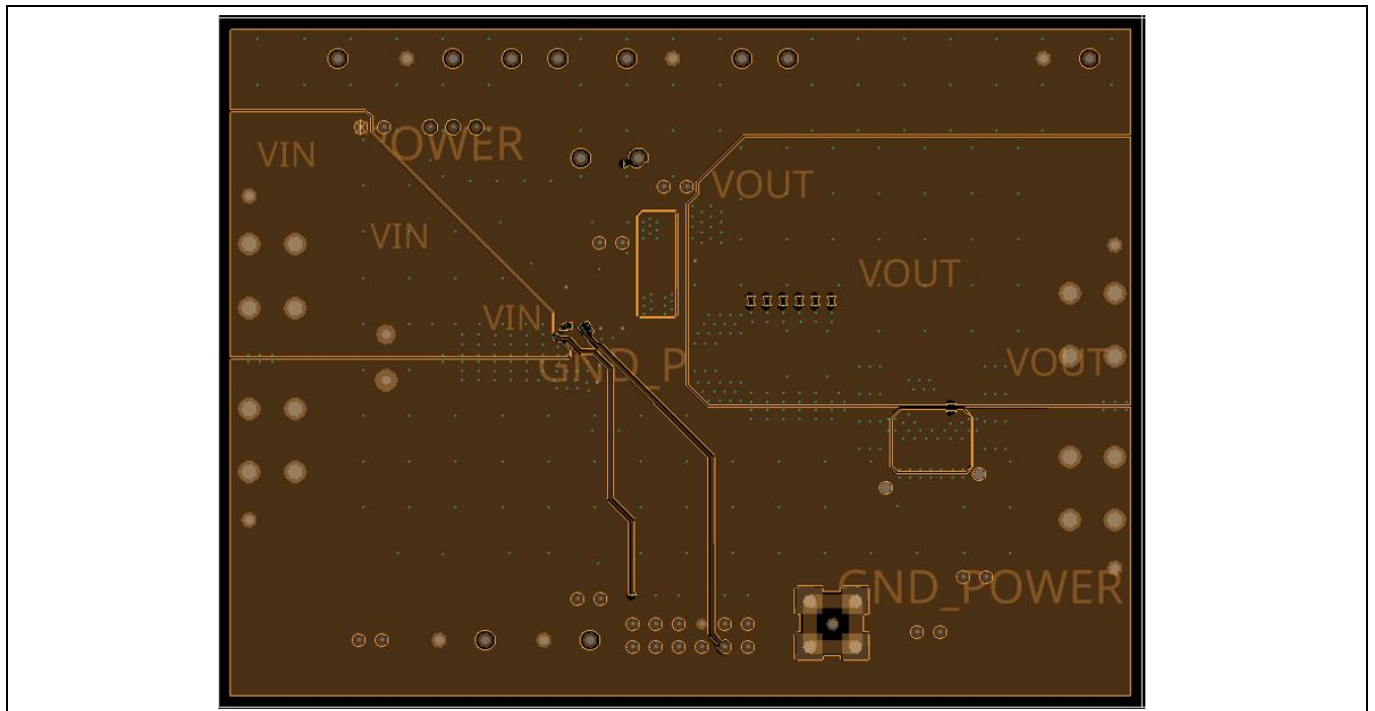
Figure 6 Inner layer 3
