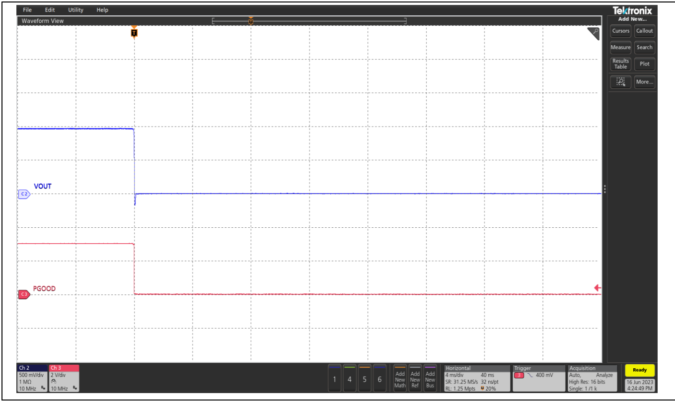
Figure 16 Short circuit and UVP (shutdown), (Ch2: V OUT , Ch3:P GOOD )
