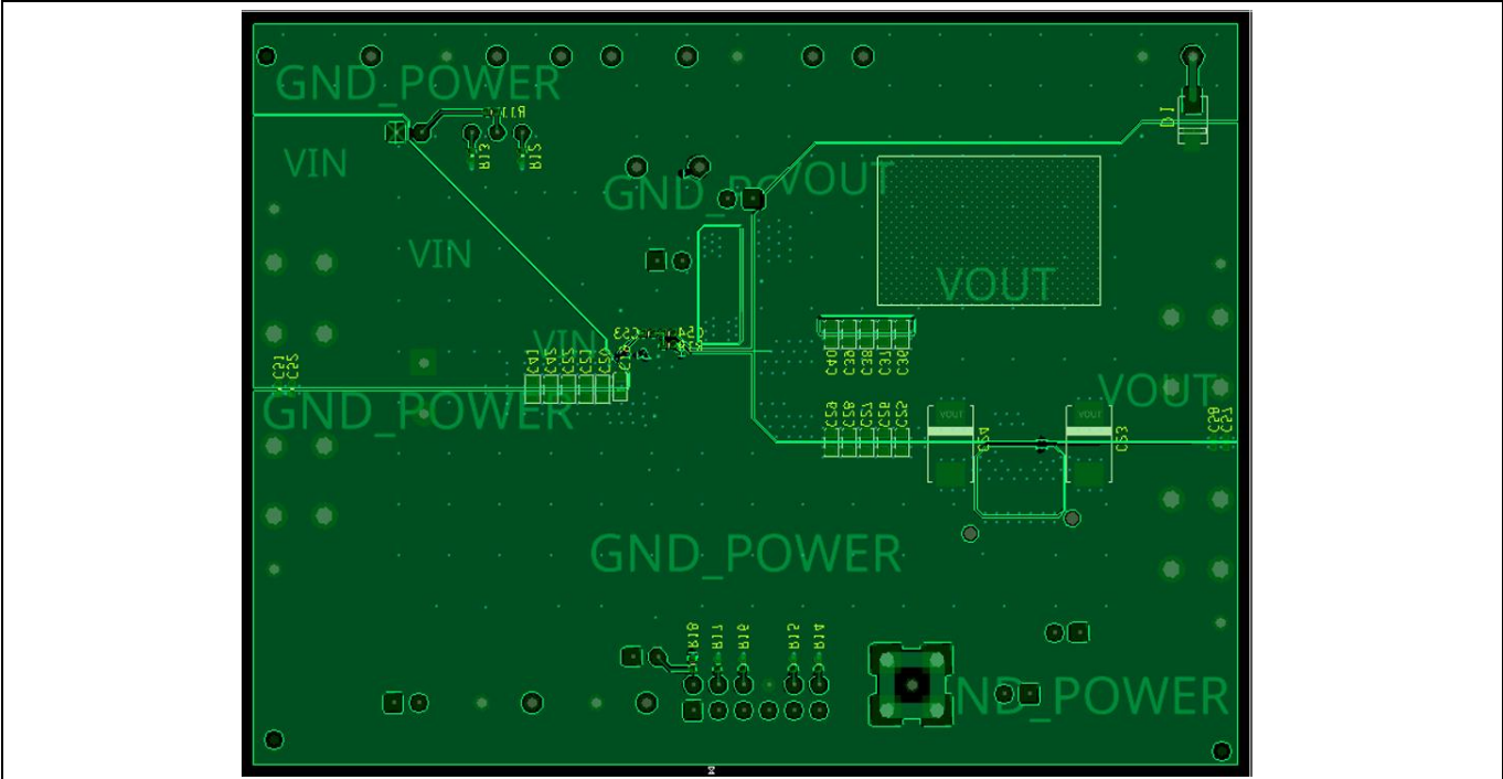
Figure 3 Bottom layer
