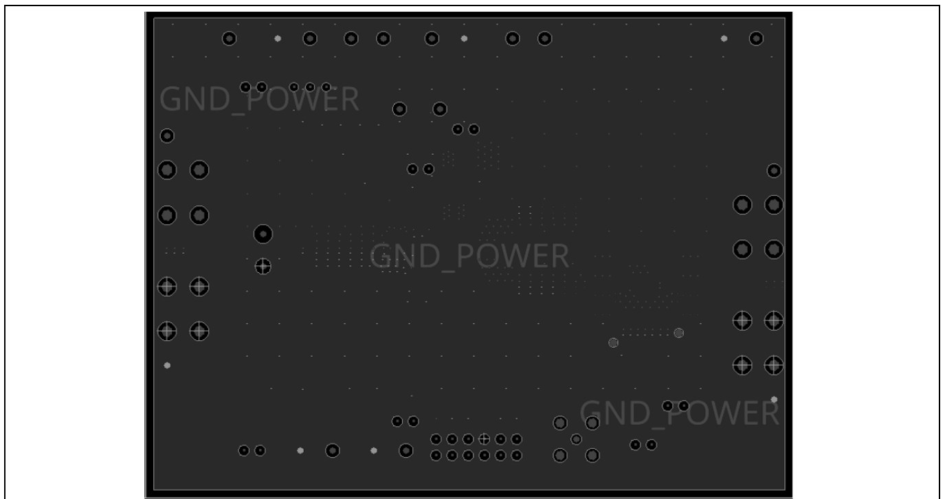
Figure 7 Inner layer 4
