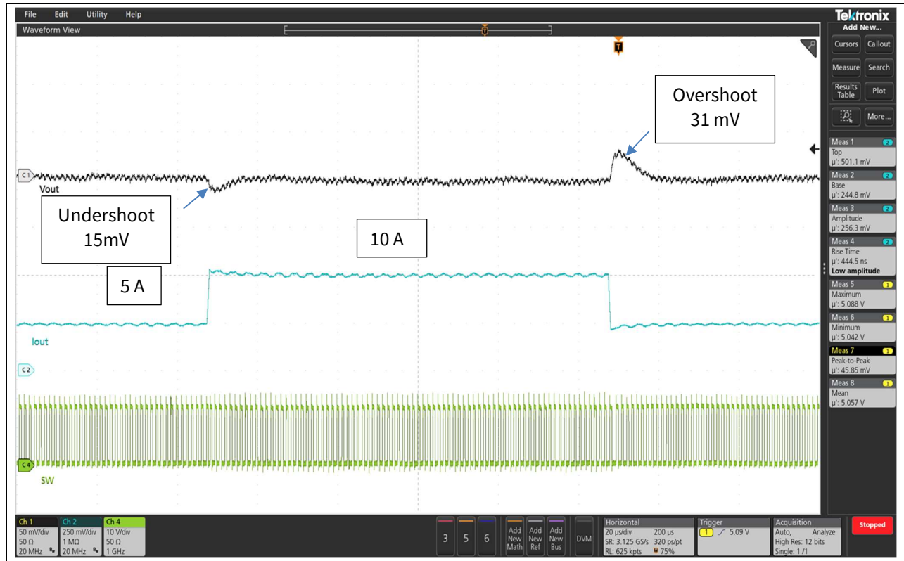
Figure 16 Transient response at 5 A step load current @ 10 A/ \mu s slew rate: I_o = 5\text{ A} - 10\text{ A} , (Ch1: V_o , Ch2: I_o , Ch4: Sw ), pk-pk: 45.85 mV, fsw = 800 kHz
