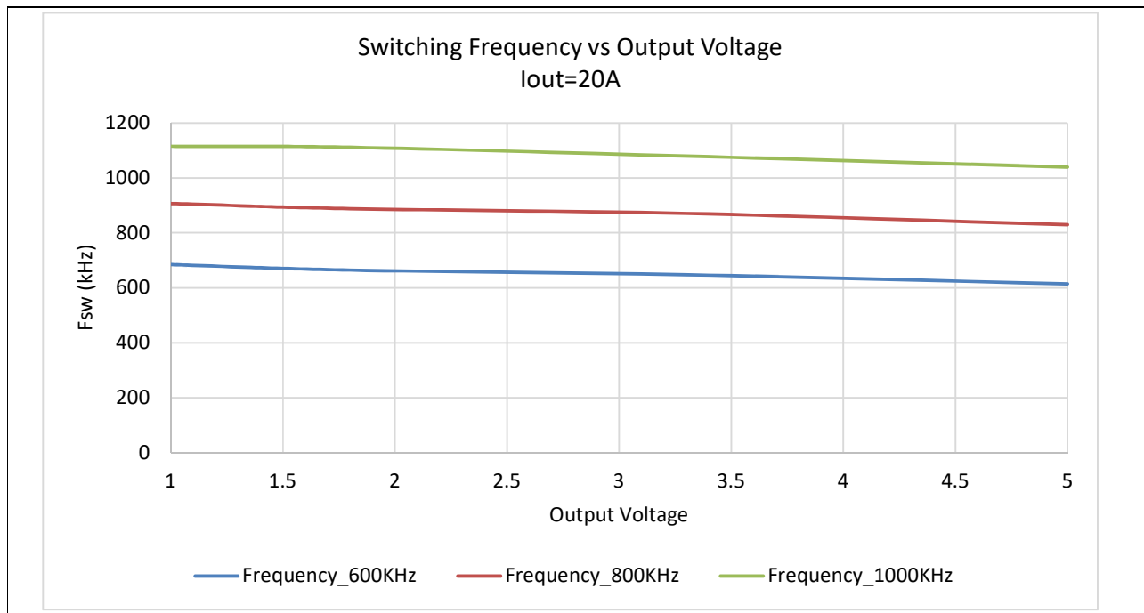
Figure 19 Switching Frequency vs Output Voltage
