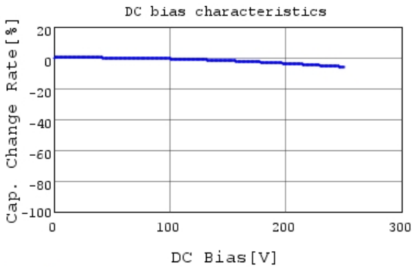
GA355DR7GF472KW01 C-DC bias capchange, 25.0c
