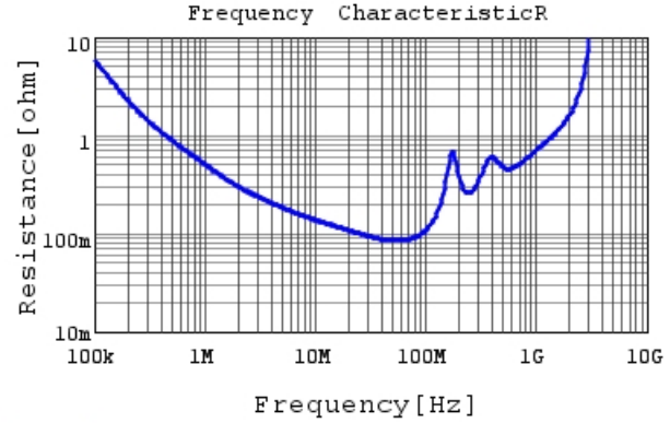
GA355DR7GF472KW01 R DCOV,25degC
