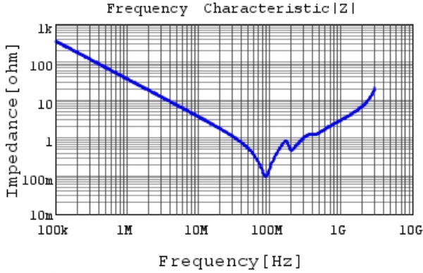
GA355DR7GF472KW01 |Z| DCOV,25degC
