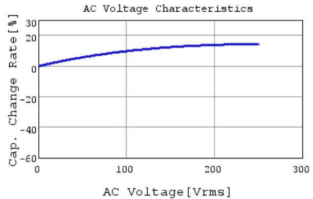
GA355DR7GF472KW01 C-AC Voltage capchange, Dc
