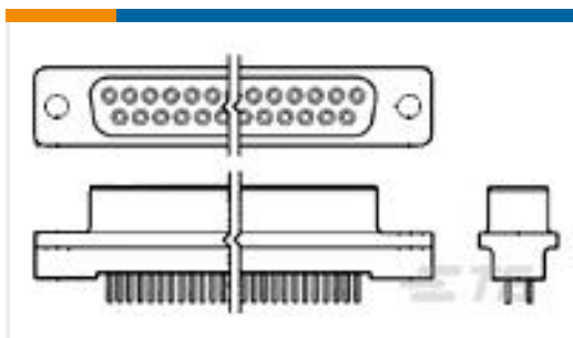
TE Part #5745076-4 HD-20 RCPT 9P VERT FFSCRLK
