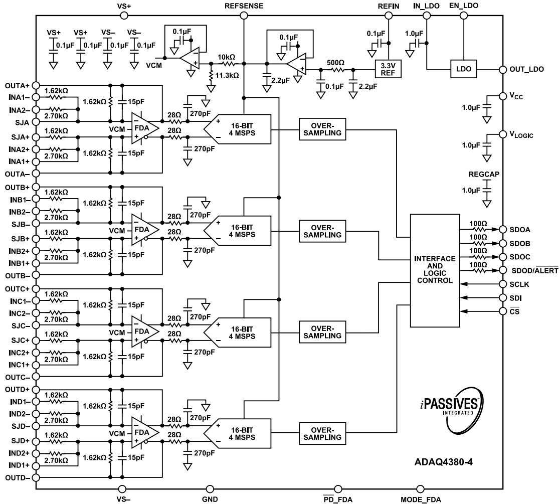
Figure 46. ADAQ4380-4 μModule Simplified Block Diagram
