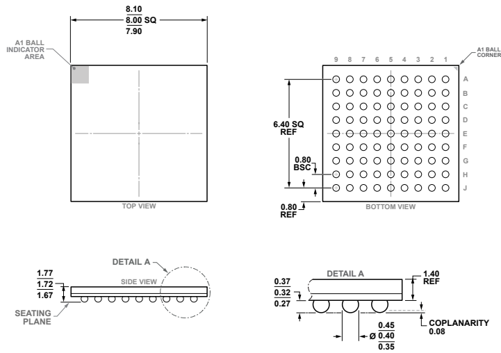
Figure 79. 81-Ball Chip-Scale Package Ball Grid Array [CSP_BGA] (BC-81-7) Dimensions Shown in millimeters
