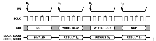
Figure 76. Register Write
