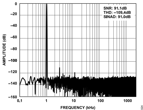
Figure 24. 1 kHz, -0.5 dBFS Input tone FFT, Gain = 0.3, Differential Input, Low Power
