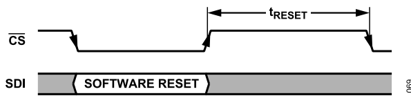
Figure 69. Software Reset Operation
