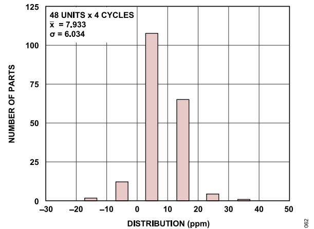
Figure 62. Reference Output Voltage Hysteresis at Four Full Cycles
