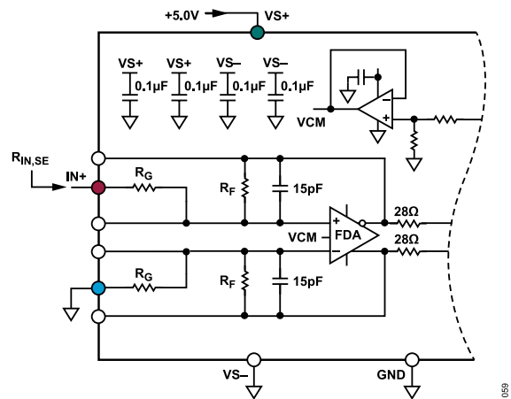
Figure 59. ADAQ4380-4 Configured at Single-Ended Inputs
