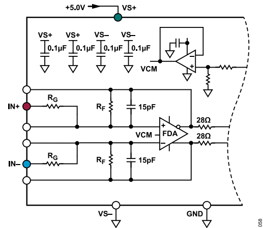
Figure 58. ADAQ4380-4 Configured at Fully Differential Inputs
