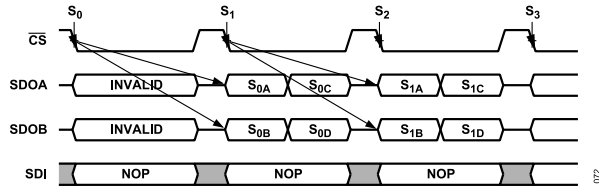
Figure 72. Reading Conversion Results, 2-Wire Mode
