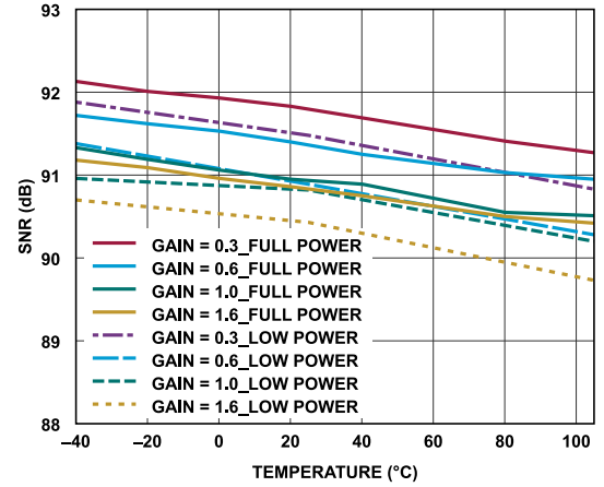
Figure 37. SNR vs. Temperature, f_{IN} = 1 \text{ kHz}
