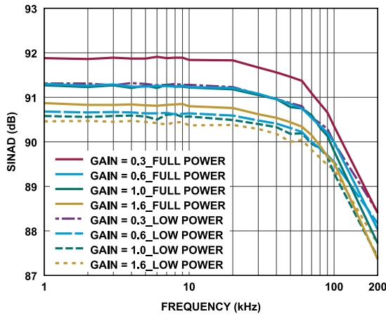
Figure 36. SINAD vs. Frequency
