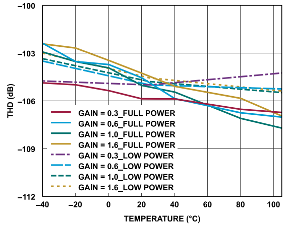
Figure 38. THD vs. Temperature, f_{IN} = 1 \text{ kHz}
