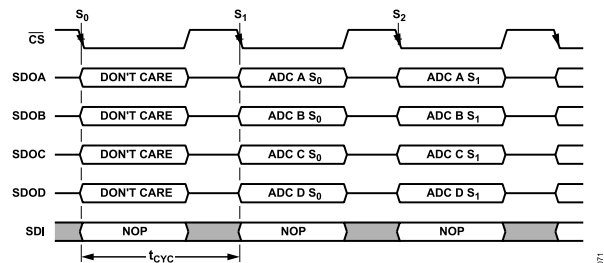
Figure 71. Read Conversion Results, 4-Wire Mode
