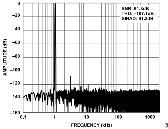
Figure 28. 1 kHz, -0.5 dBFS Input tone FFT, Gain = 0.6, Differential Input, Full Power
