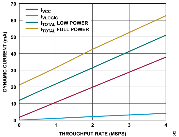
Figure 42. Dynamic Current vs. Throughput Rate
