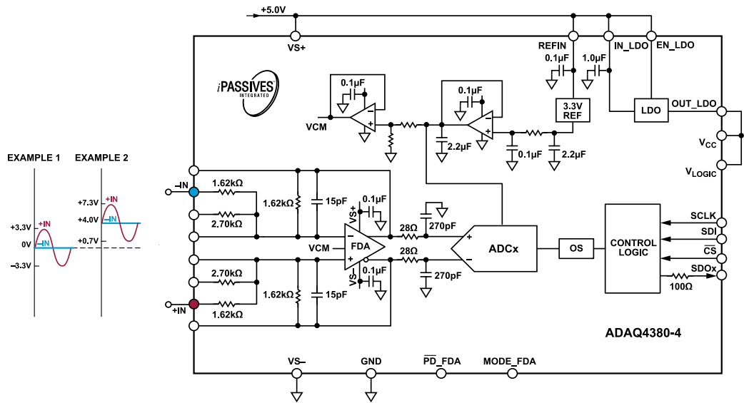
Figure 54. Single-Ended Input Configuration with Gain = 1.0, ±3.3 V Input, V_S = 5\text{ V}
