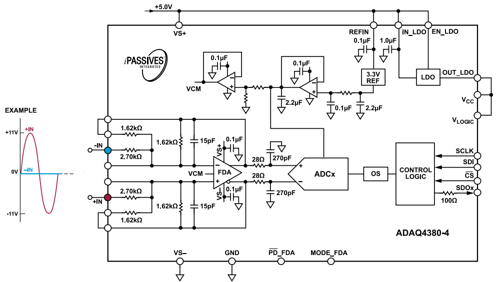
Figure 52. Single-Ended Input Configuration with Gain = 0.3, ±11 V Input, V_S = 5\text{ V}
