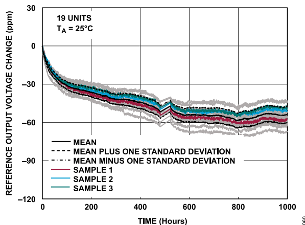
Figure 60. ADAQ4380-4 Internal Reference Long-Term Drift
