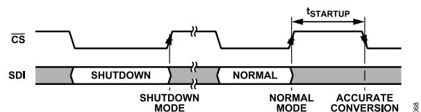
Figure 68. Shutdown Mode Operation
