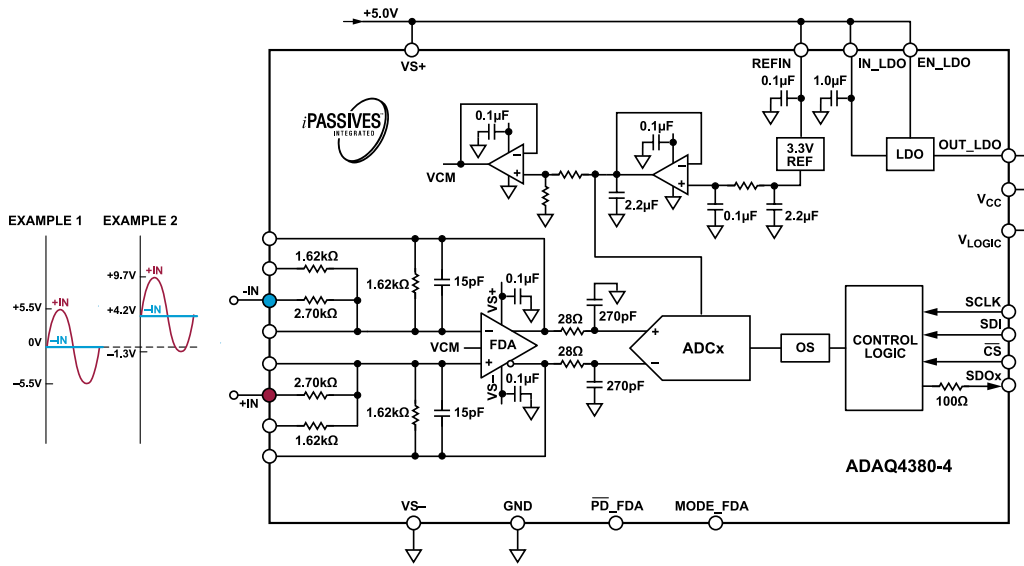
Figure 53. Single-Ended Input Configuration with Gain = 0.6, ±5.5 V Input, V_S = 5\text{ V}
