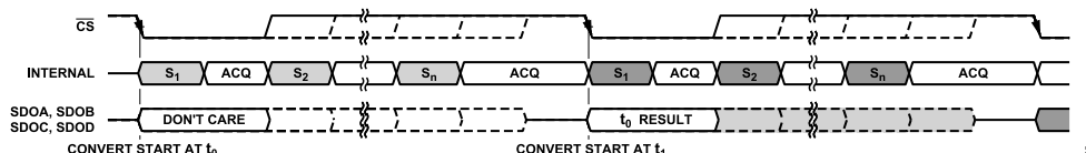
Figure 65. Normal Average Oversampling Operation
