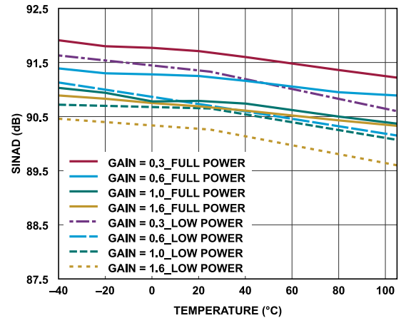
Figure 39. SINAD vs. Temperature, f_{IN} = 1 \text{ kHz}
