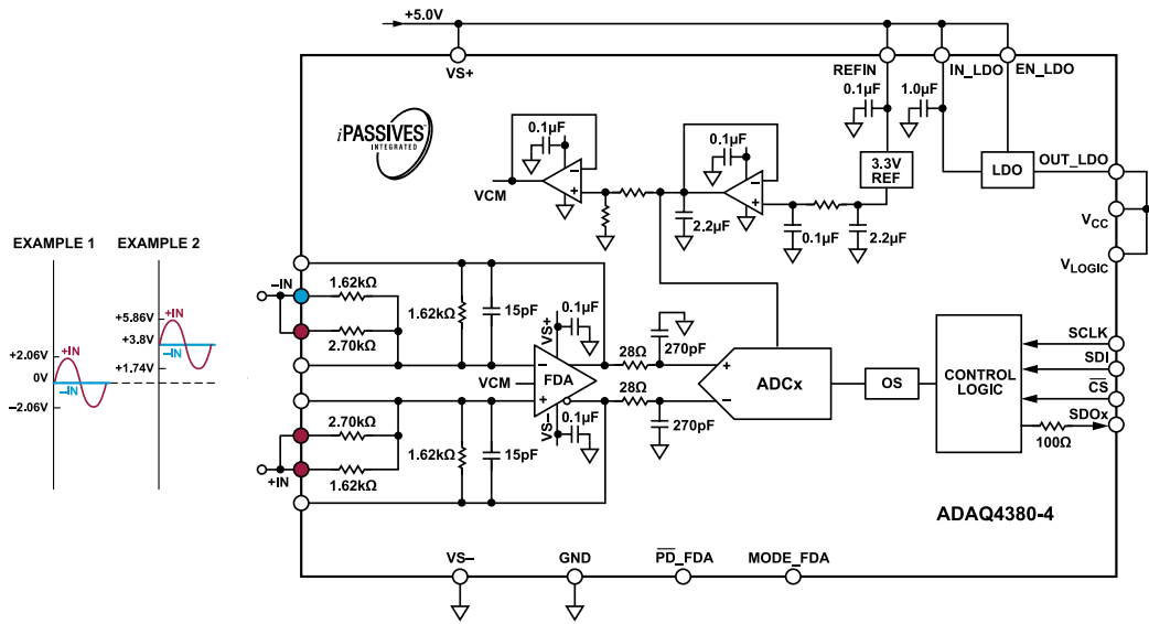
Figure 55. Single-Ended Input Configuration with Gain = 1.6, ±2.06 V Input, V_S = 5\text{ V}
