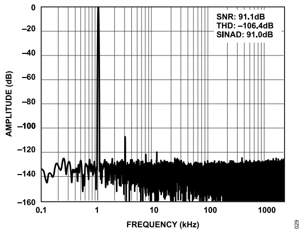
Figure 29. 1 kHz, -0.5 dBFS Input tone FFT, Gain = 1.0, Differential Input, Full Power
