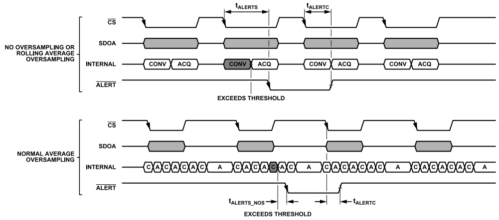
Figure 8. ALERT Timing
