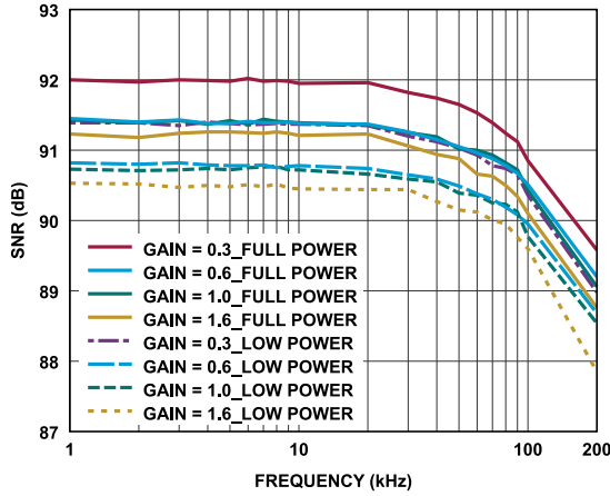
Figure 34. SNR vs. Frequency
