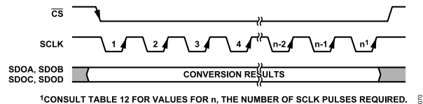
Figure 70. Reading Conversion Results
