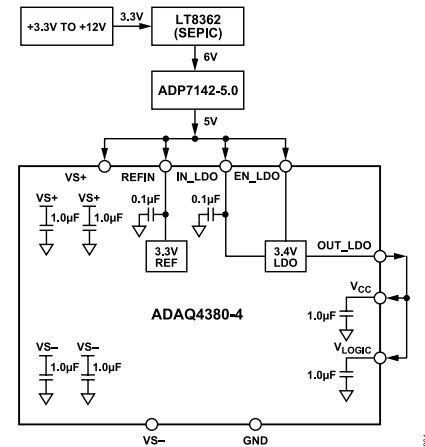
Figure 64. ADAQ4380-4 Power Supply Recommendations
