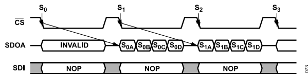
Figure 73. Read Conversion Results, 1-Wire Mode
