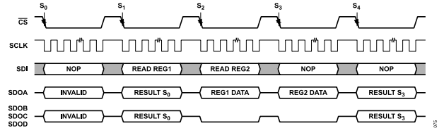
Figure 75. Register Read
