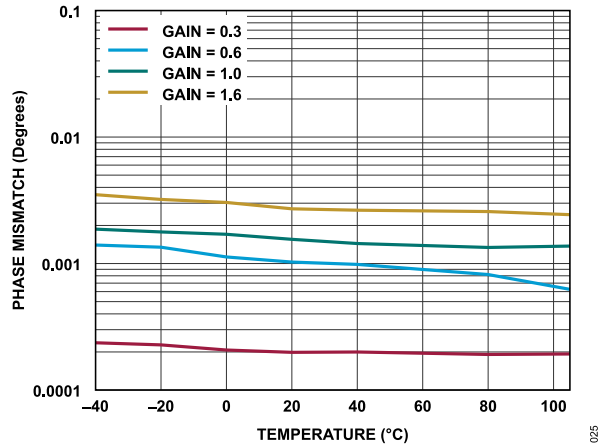
Figure 25. Channel-to-Channel Phase Matching vs. Temperature, f_{IN} = 20 \text{ kHz}
