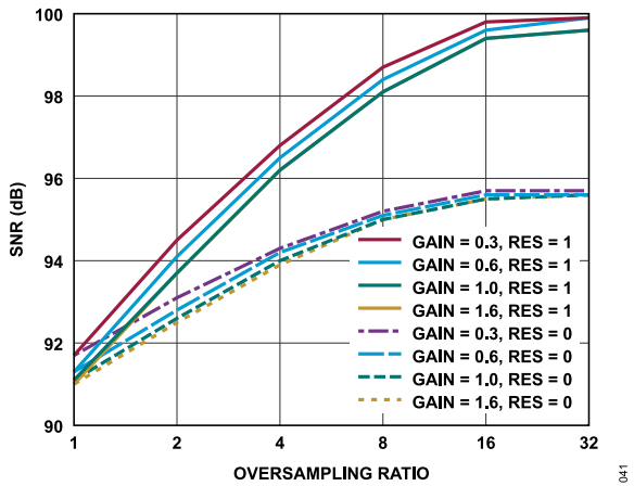
Figure 41. SNR vs. Normal Average Oversampling, f_{IN} = 1 \text{ kHz}
