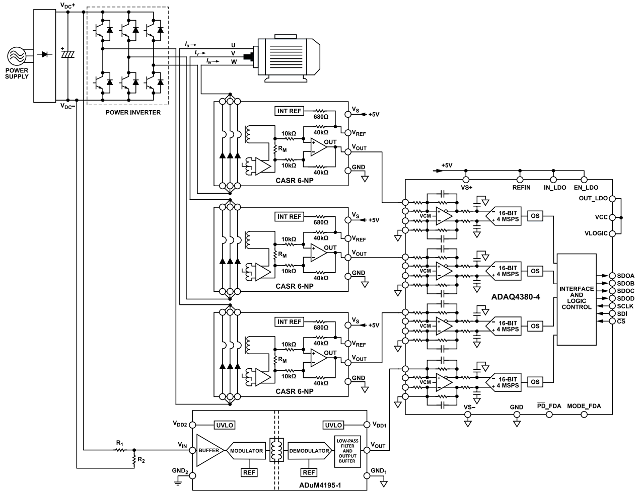
Figure 1. Precision Current and Voltage Sensing for Servo Motors Control
