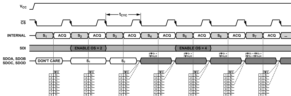
Figure 66. Rolling Average Oversampling Mode Operation
