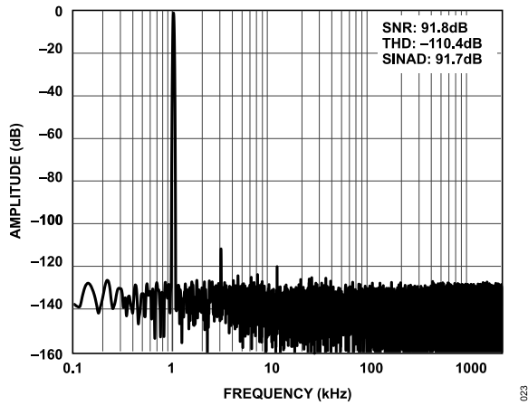
Figure 23. 1 kHz, -0.5 dBFS Input tone FFT, Gain = 0.3, Differential Input, Full Power
