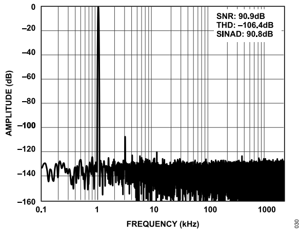
Figure 30. 1 kHz, -0.5 dBFS Input tone FFT, Gain = 1.6, Differential Input, Full Power
