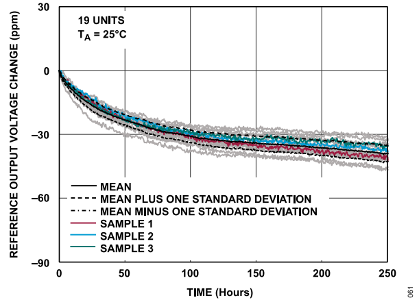
Figure 61. ADAQ4380-4 Internal Reference Early Life Drift
