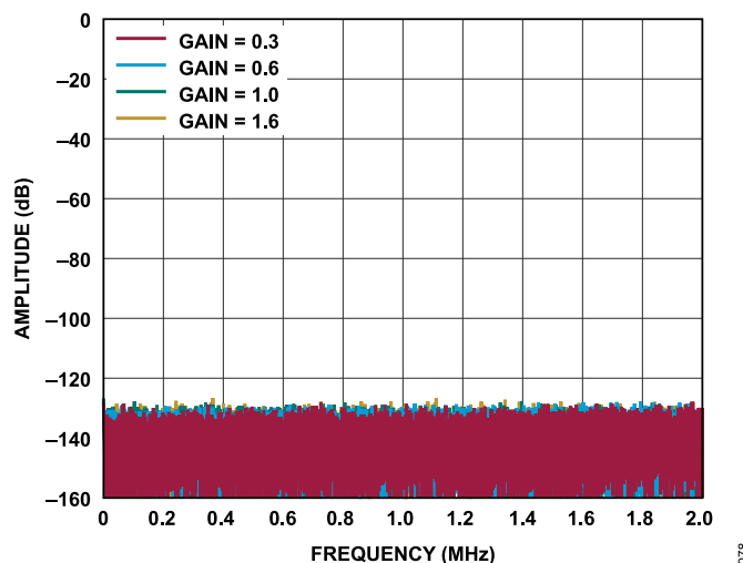
Figure 78. FFT with Shorted Inputs
