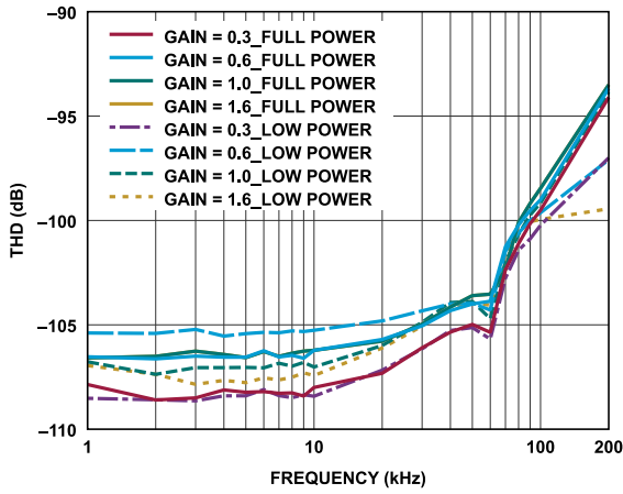
Figure 35. THD vs. Frequency
