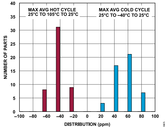
Figure 63. Reference Output Voltage Hysteresis at Half Cycles
