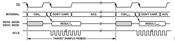
Figure 74. Low Throughput and Low Latency
