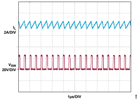
Figure 8. Switching Waveforms, Full-Frequency PWM Operation. V_{IN} = 6V , I_{LOAD} = 900mA
