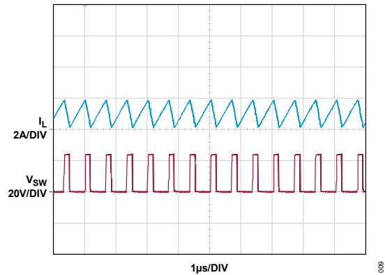
Figure 9. Switching Waveforms, Continuous Burst Mode Operation. SYNC/MODE = 0V , V_{IN} = 6V , I_{LOAD} = 230mA
