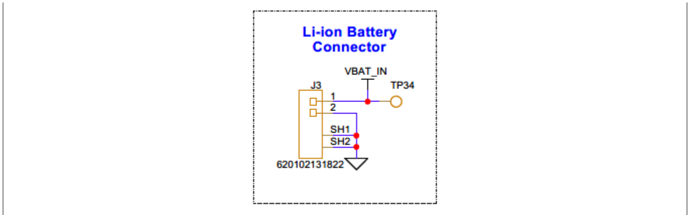
Figure 13 Schematic of power supply inputs of evaluation kit
