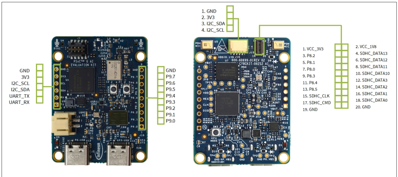
Figure 2 Board pinout
