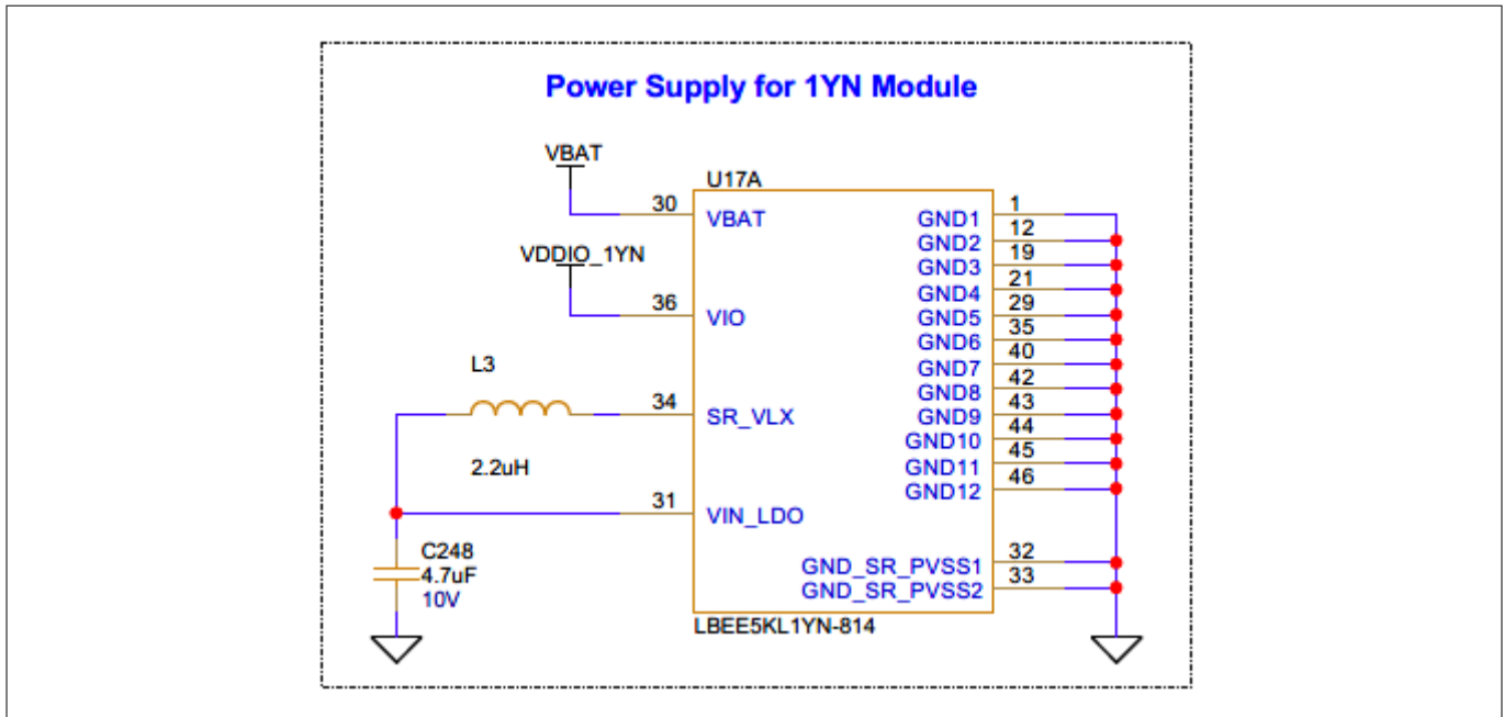
Figure 39 1YN module power supply schematic
