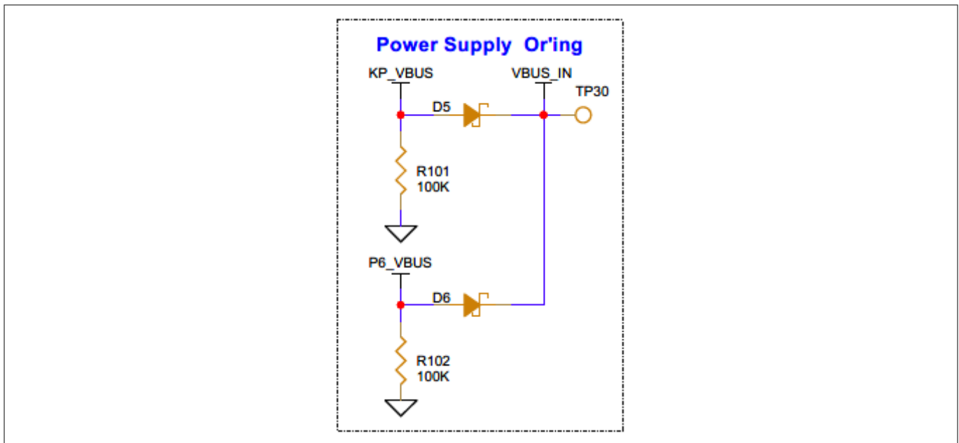
Figure 14 Schematic of power supply Or'ing
