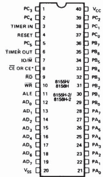
231719-2 Figure 2. Pin Configuration
