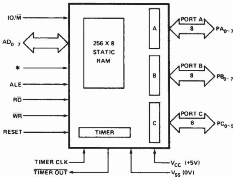
*8155H/8155H-2 = \overline{CE} , 8156H/8156H-2 = CE 231719-1 Figure 1. Block Diagram
