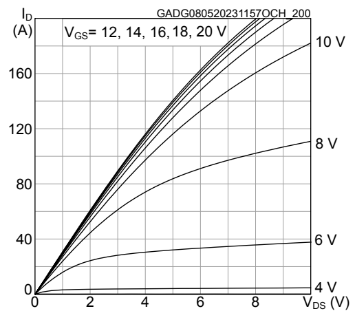
Figure 4. Typical output characteristics ( T_J = 200\text{ }^\circ\text{C} )
