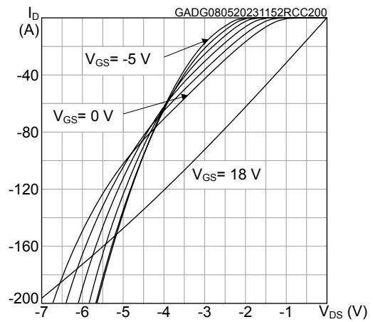
Figure 16. Typical reverse conduction characteristics ( T_J = 200 \text{ °C} )
